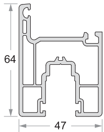
Sliding Window Sash Code No : DP - 703
