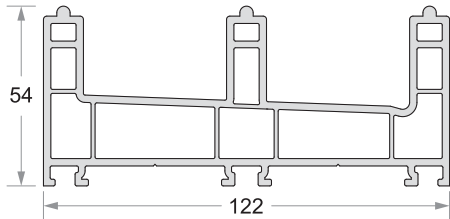
3 Track Sliding Frame Code No : DP - 702
