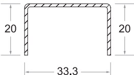
Window Sash Code No : ST - 703
