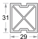
Reinforcement Code No : DPDR - 3129
