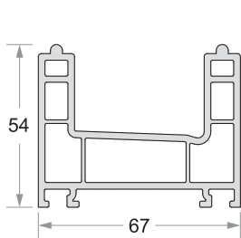
2 Track Sliding Frame Code No : DP - 701
