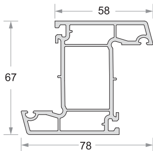
'Z' Mullion Code No : DP - 753
