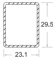
False Mullion Code No : ST - 757
